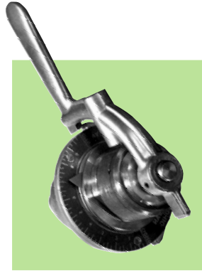
1813 Sensitrol Valve on a Dual-Fuel™ burner. Valve is used for setting ratio when burner is on oil; it is shut off when burning gas.
